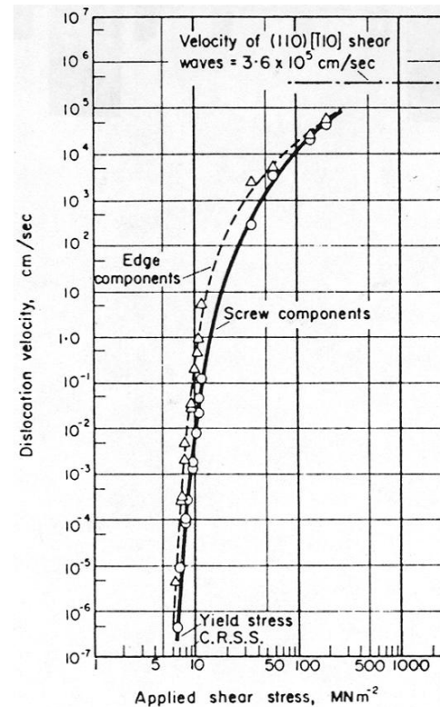
(a) Stress dependence of the velocity of edge and screw dislocations in lithium fluoride. (From Johnston and Gilman, J. Appl. Phys. 30, 129, 1959.)
